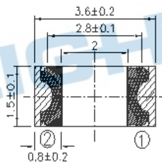
Recommend Soldering Pad
