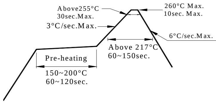
3.1 Pb-free solder temperature profile
