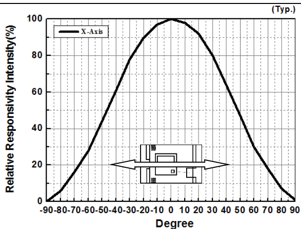
Fig.5 View Angle (X-axis)
