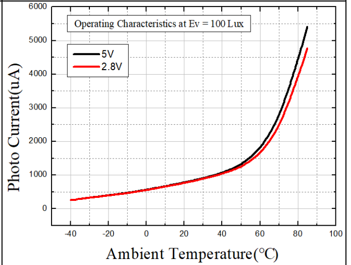
Fig.8 Photo Current vs. Ambient Temperature
