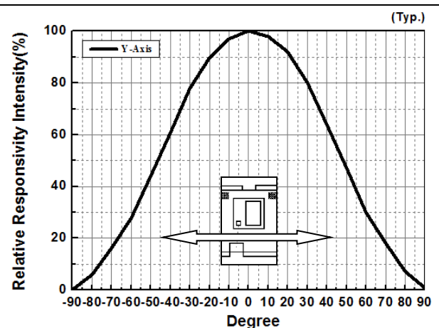
Fig.6 View Angle (Y-axis)
