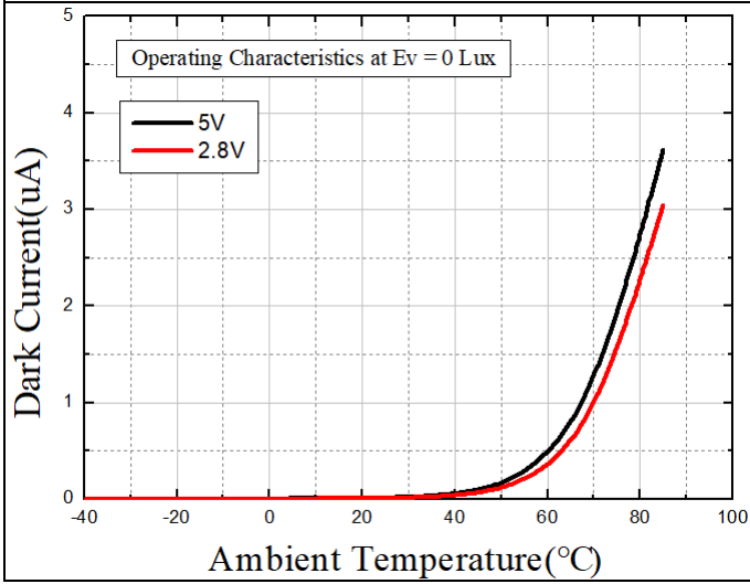
Fig.7 Dark Current vs. Ambient Temperature
