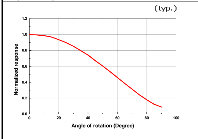
Fig.7 Angular response
