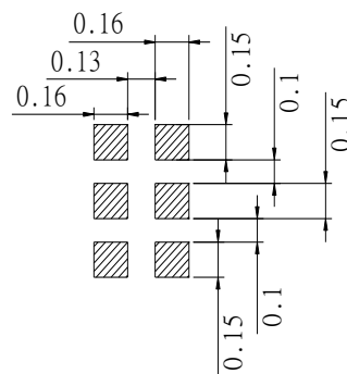
Soldering patterns
