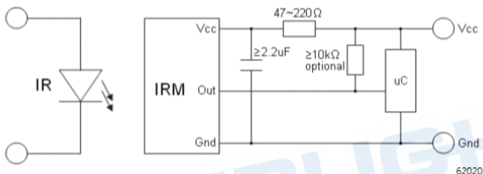
Fig.9: application circuit
