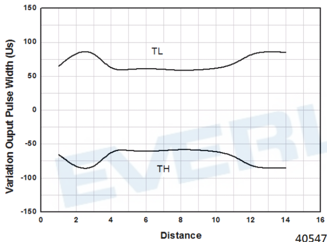
Fig.6 Variation Ouput Pulse Width VS. Distance
