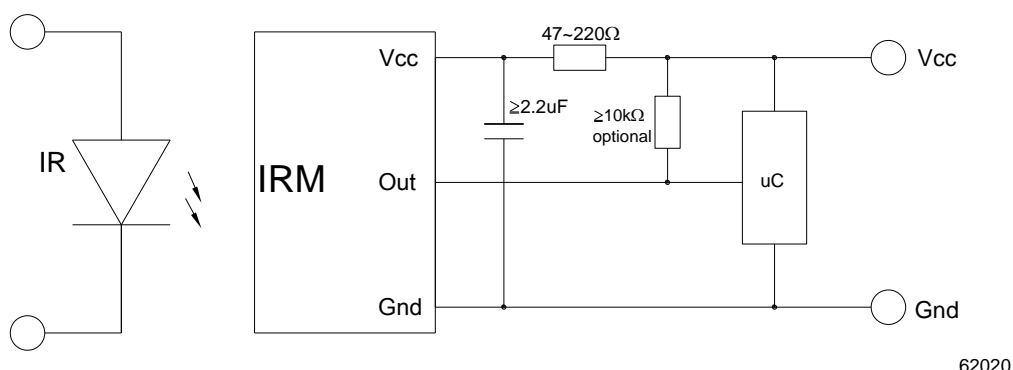
Fig.9: application circuit
