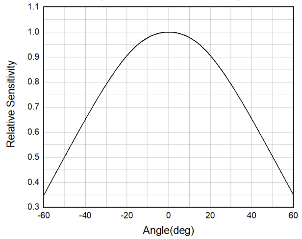
Fig.5 Relative Sensitivity vs. Angle
